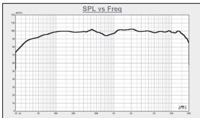
Amplitude vs. Frequency Response of the Radian 1312NEO as measured on axis with a one watt (2.83 Vrms), swept sine wave input at 8 ohms, using a 324/12 crossover network in a 2.3 (ft. 3 ) vented cabinet.
